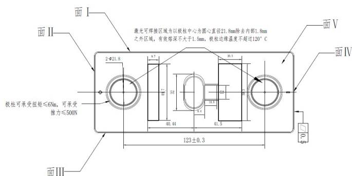
二维图纸 2D Drawing
